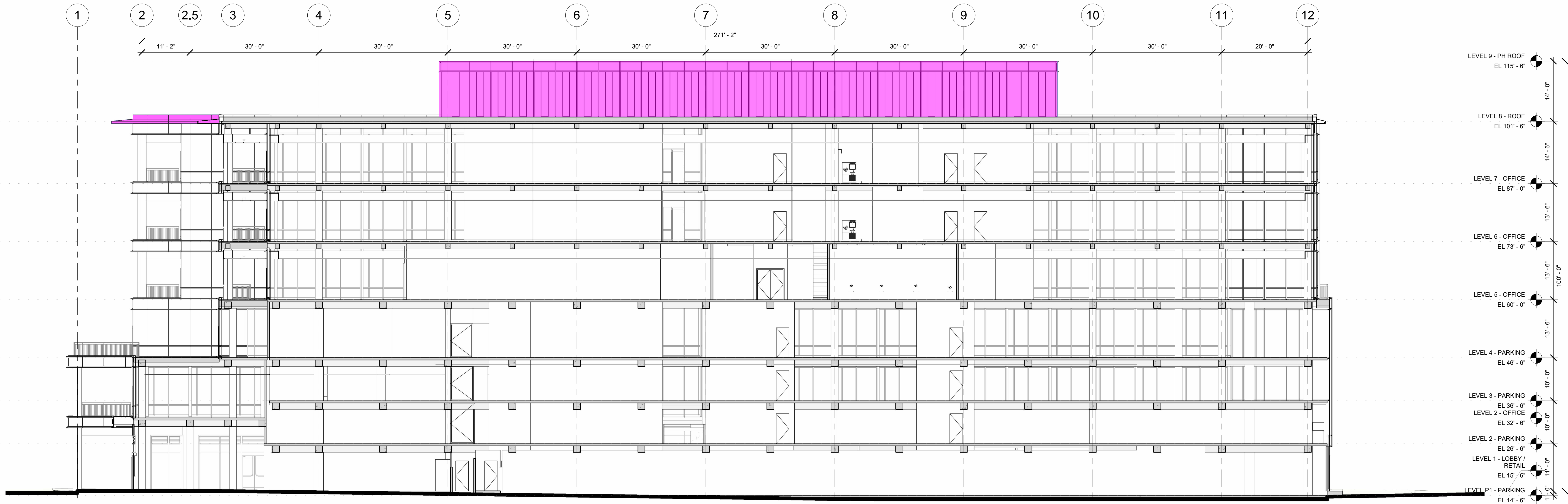
1 E-W BUILDING SECTION - A 3/32" = 1'-0"
